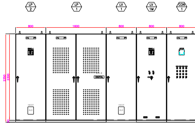
저압반 FRONT VIEW
