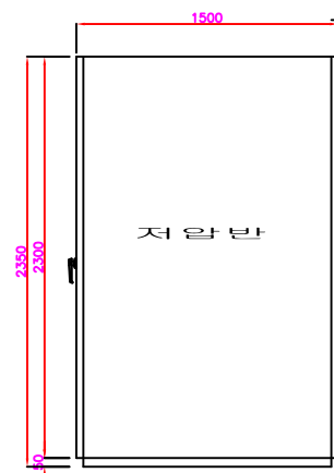
저압반 SIDE VIEW
